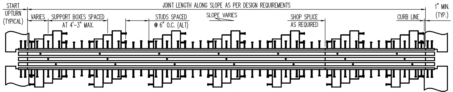
TYPICAL 'D-320' PLAN VIEW
