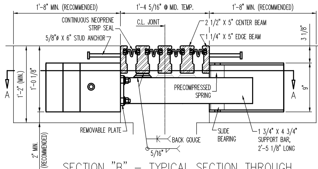
SECTION "B" - TYPICAL SECTION THROUGH 'D-320' EXPANSION JOINT @ SUPPORT BOX
