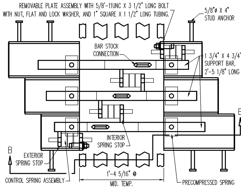
DETAIL "A" - PLAN VIEW OF 'D-320' EXPANSION JOINT @ SUPPORT BOX
